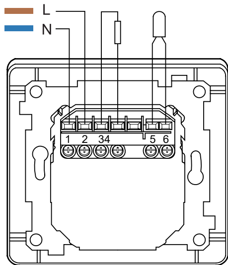
Schlüter®-DITRA-HEAT-E-R /-R-WIFI
