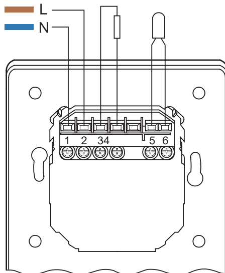
Schlüter®-DITRA-HEAT-E-R /-R3
