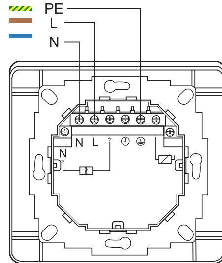
Schlüter®-DITRA-HEAT-E-R /-R4
